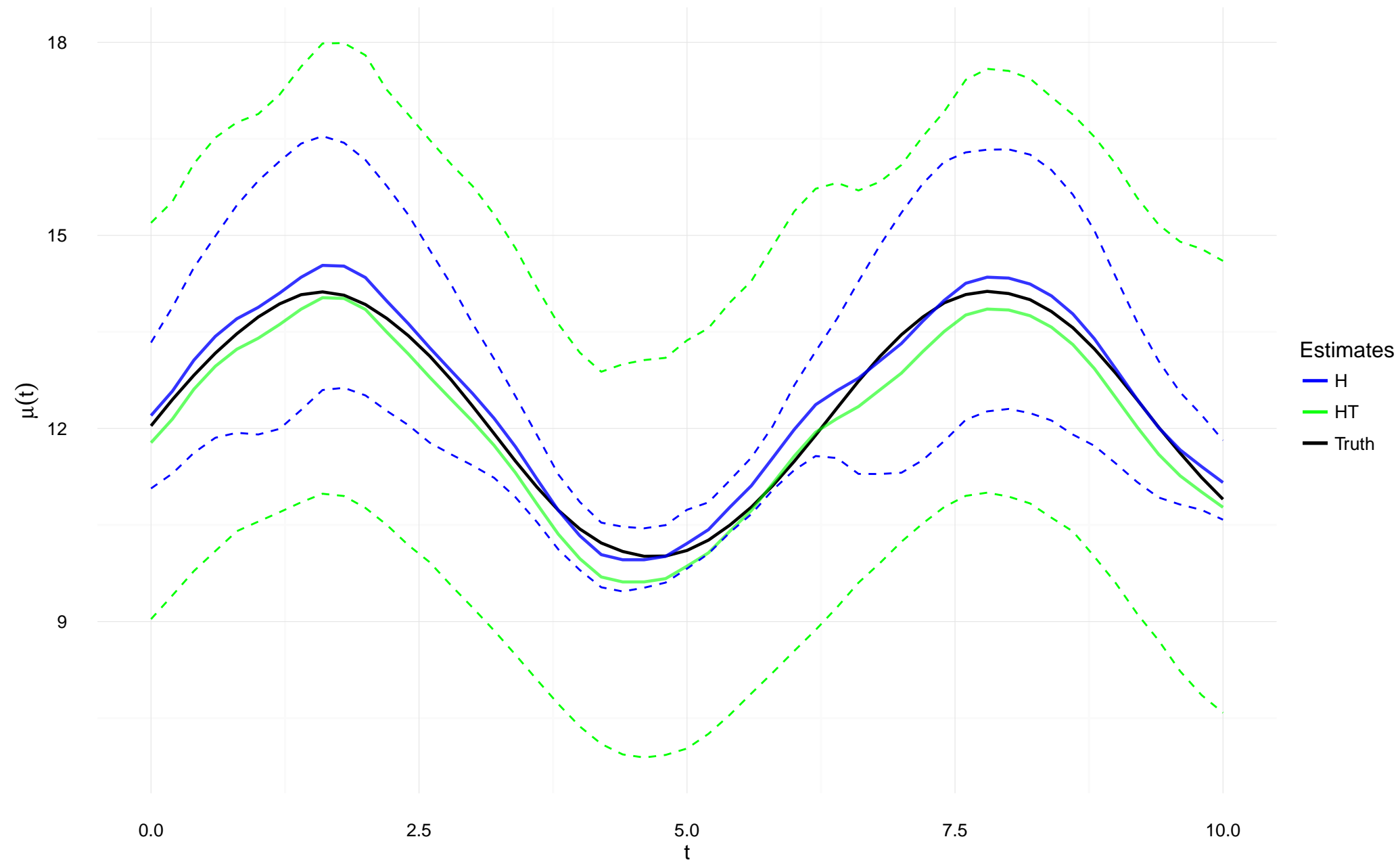
Confidence Bands
